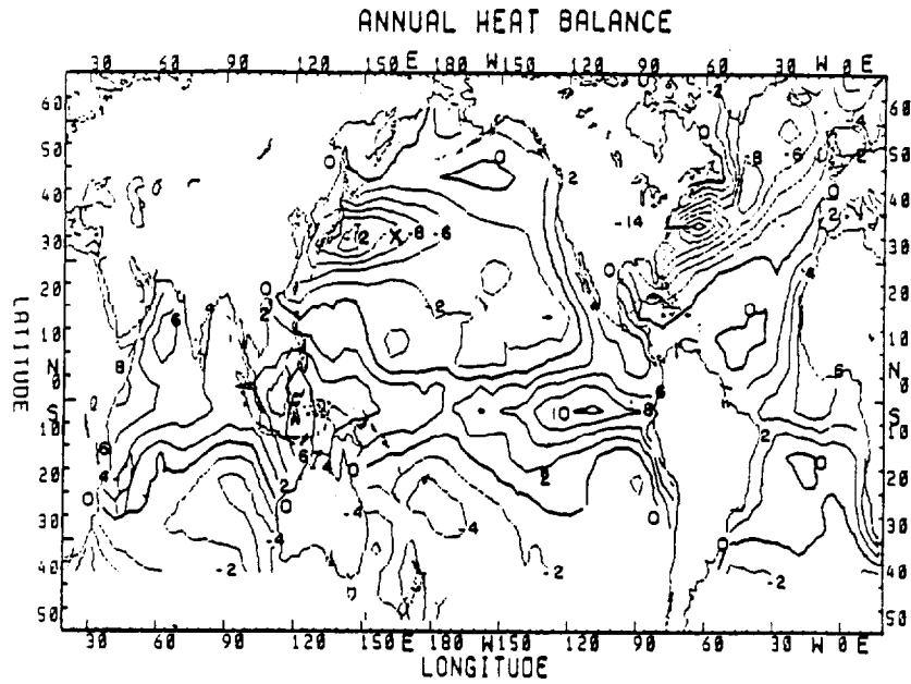
Figure 4. Annual mean net heat balance at the surface. The units are in W m^{-2} when multiplied by 10. (from Hsiung 1985) The cross at 35^{\circ}N, 165^{\circ}E shows the position of heat estimate in Fig. 5
