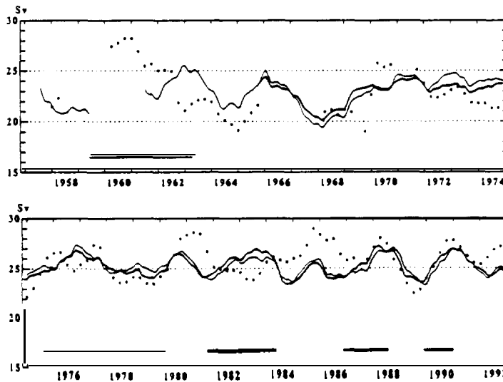
Figure 3. Interannual variations of volume transport of the Kuroshio in the East China Sea, by geostrophic calculation (dots) and estimated from tide gauge data fitted to the geostrophic transports (lines). The horizontal lines show the large meander periods. (from Kawabe 1995)
