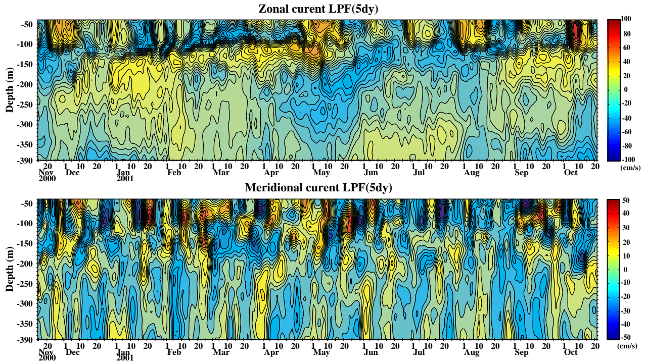
Figure 2: Time-depth sections of the zonal and meridional currents at 90°E on the equator. Five-day low-passed filter was applied to the original data.
