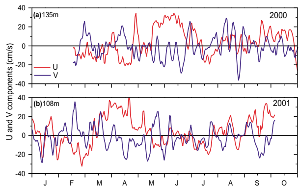
Figure 3: Temporal variation of Zonal & Meridional components (de-tided and daily averaged) at first level from current meter moorings at equator, 93°E during January-October 2000 and 2001
